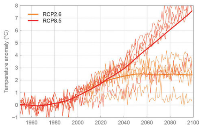
Figure 5.3: Temperature projections for the European and Central Asian region, compared to the 1951–1980 baseline for the multi-model mean (thick line) and individual models (thin lines) under RCP2.6 (2°C world) and RCP8.5 (4°C world) for the months of JJA.
