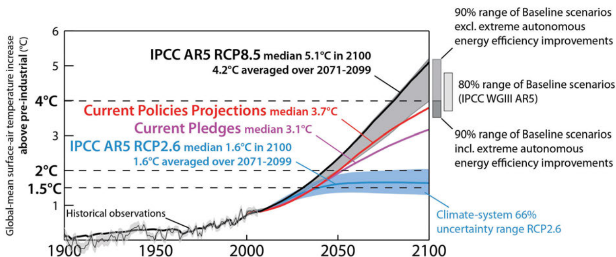
Figure 2.1: Projections for surface-air temperature increase, showing the scenarios assessed in this report in the context of baseline projections (no further substantial climate policy from the recent energy-economic model literature).
