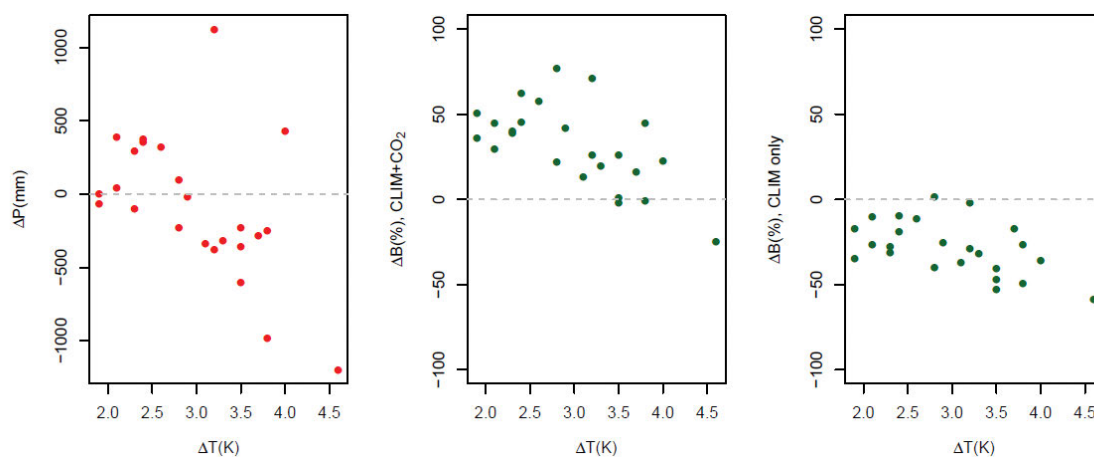
Figure 3.20: Simulated precipitation changes in Eastern Amazonia from the 24 IPCC-AR4 GCMs with regional warming levels of 2–4.5 K (left panel). Simulated changes in biomass from LPJmL forced by the 24 IPCC-AR4 climate scenarios assuming strong CO 2 fertilization effects (middle panel, CLIM+CO 2 ) and no CO 2 fertilization effects (CLIM only, right panel).
