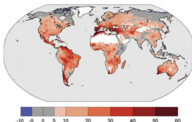
Figure 2.8: Percentile change in the occurrence of days under drought conditions by the end of the 21st century (2070–2099) in a 4°C world relative to the 1976–2005 baseline.
