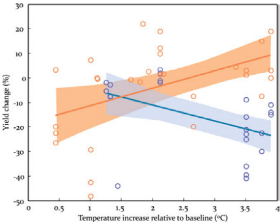
Figure 3.19: Meta-analysis of crop yield reductions.
