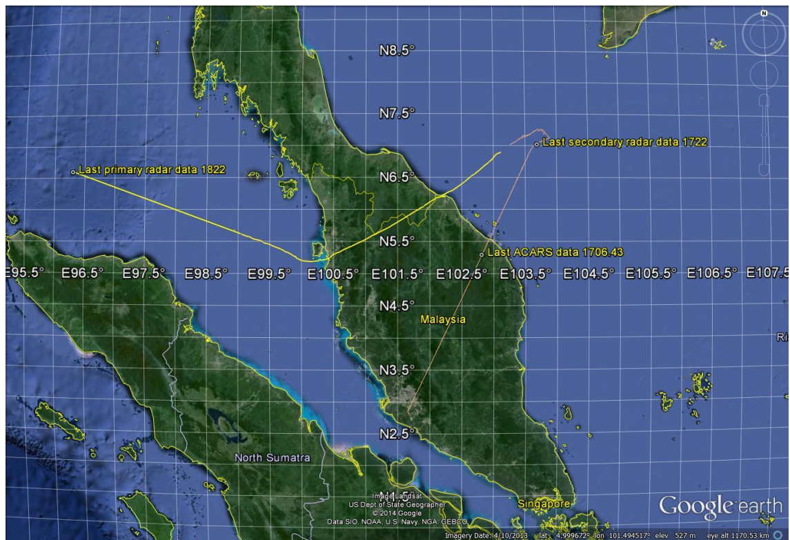
Figure 2: MH370 flight path derived from primary and secondary radar data
