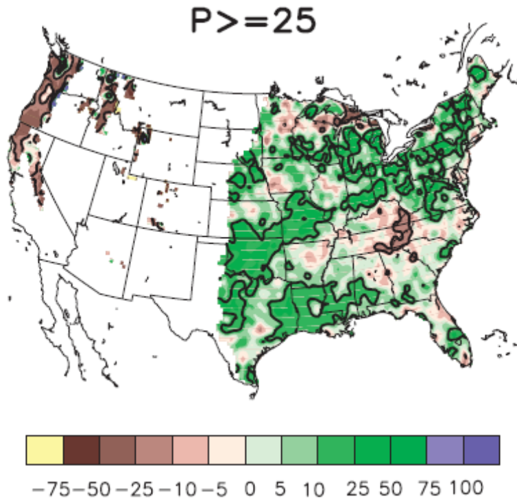
CAPTION: The percent change in the annual number of daily precipitation events (1980-2009 minus 1950-79) for daily events which produced over 25mm of precipitation (from Higgis and Kousky, 2013).
