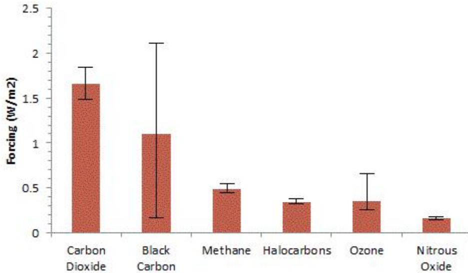
CAPTION: Relative warming influence of the major anthropogenic emissions (whiskers are the 90% uncertainly bounds) (from IPCC AR4, and Bond et al., 2013).
