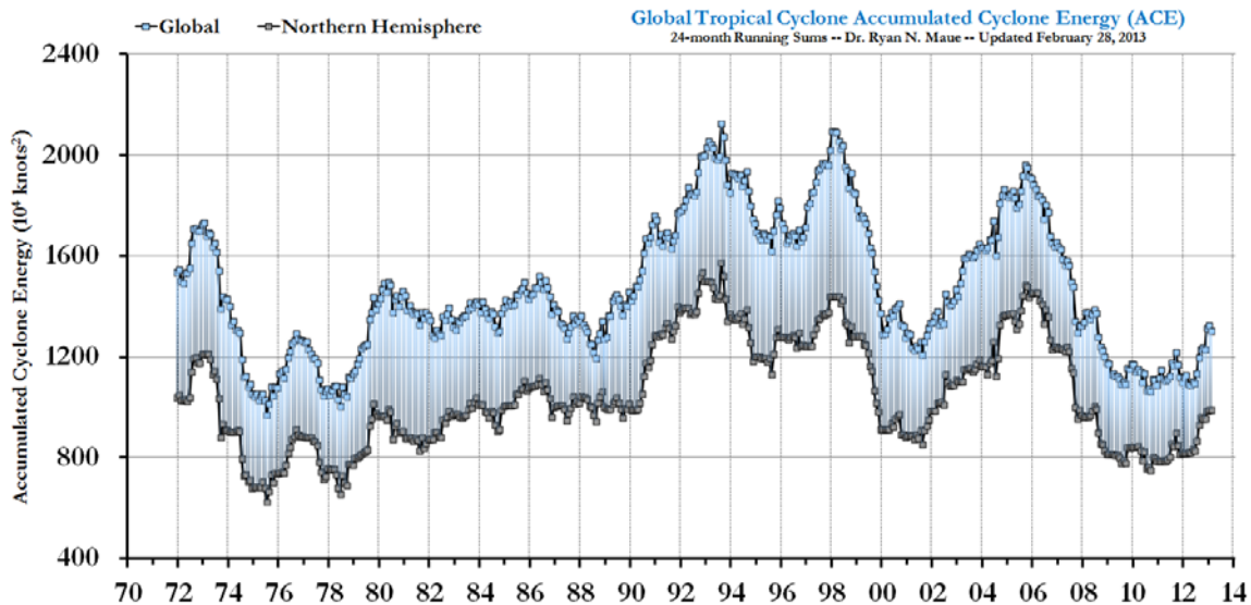
CAPTION: Last 4-decades of Global and Northern Hemisphere Accumulated Cyclone Energy: 24 month running sums. Note that the year indicated represents the value of ACE through the previous 24-months for the Northern Hemisphere (bottom line/gray boxes) and the entire global (top line/blue boxes). The area in between represents the Southern Hemisphere total ACE. (data source: updates from Maue et al., 2011)
