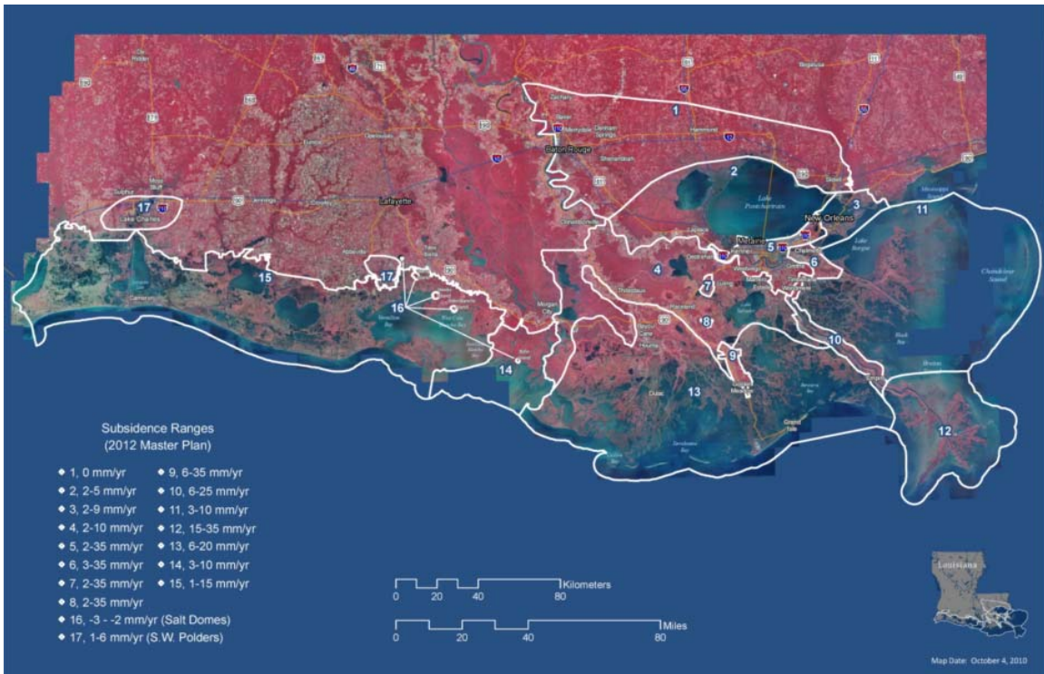
CAPTION: This map shows an estimate of the rate of land subsidence along the Louisiana coast—a sinking of the land not related to global sea level rise. Although the subsidence rate varies by a large amount along the Louisiana coastline, on average it is occurring at a rate about 5 times greater than the actual sea level is rising. What this means, is that in most areas along the Louisiana coast will experience sea level rise close to 4 feet from land sinking alone and irrespective of global warming-induced sea level rise. Therefore actions to mitigate the impact of a large sea level rise will be required, where necessary, from ongoing changes in the geography of the region. (figure from: Recommendations for Anticipation sea-level rise impacts on Louisiana Coastal Resources during Project Planning and Design. Draft report, 2012, Louisiana Applied Coastal Engineering and Science (LACES) Division, Coastal Protection and Restoration Authority of Louisiana, State of Louisiana. http://coastal.louisiana.gov/index.cfm?md=pagebuilder&tmp=home&pid=240 )
