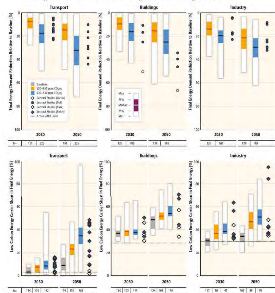
Figure 4.3: Final energy demand reduction relative to baseline (upper row) and low-carbon energy carrier shares in final energy (lower row) in the , transport, buildings, and industry sectors by 2030 and 2050 in mitigation scenarios from two different CO 2 -eq concentration categories (see Section 6.3.2) compared to sectoral studies assessed in Chapters 8-10. Low-carbon fuels include electricity, hydrogen and liquid biofuels in transport, electricity in buildings and electricity, heat, hydrogen and bioenergy in industry. The numbers at the bottom of the graphs refer to the number of scenarios included in the ranges which differs across sectors and time due to different sectoral resolution and time horizon of models. {WG III figure SPM.11}
