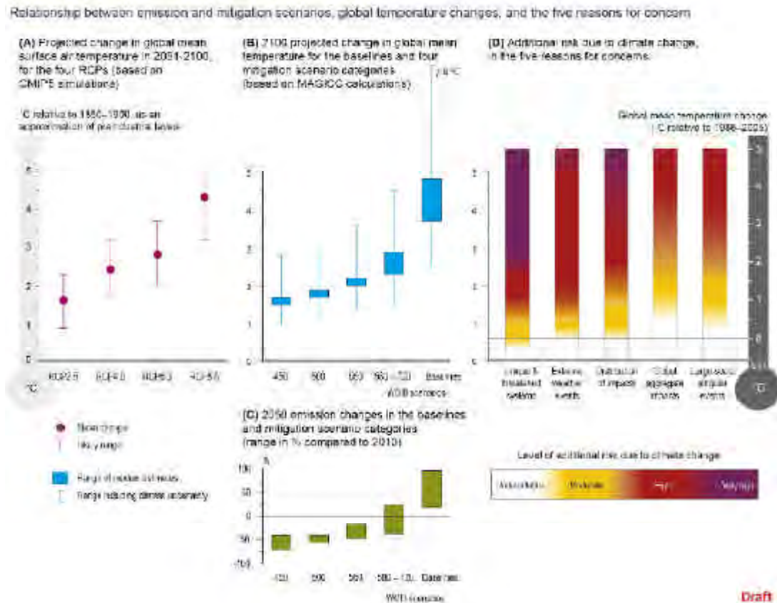
Figure 3.4: Relationship between emission and mitigation scenarios, global temperature changes, and the five Reasons for Concerns (RfC). Temperature changes shown compared with pre-industrial levels. For reference, the extreme right temperature axis shows temperature changes with respect to the 1986-2005 period. Panel a shows projected change in global temperature in 2081-2100 for the four RCPs, based on CMIP5 simulations (Table 2.1). Panel b shows the projected temperature increase in 2100, calculated using the MAGICC climate model for the baselines and four mitigation scenario categories defined in Chapter WGIII.6, indicating the uncertainty range resulting both from the range of emission scenario projections within each category and the uncertainty in the climate system {data from WGIII.6}. Panel c shows the 2050 changes in emissions in the corresponding baselines and mitigation scenario categories (positive changes refer to cases where emissions in 2050 are larger than 2010). For instance, the mitigation scenarios in the 450 category – i.e. with CO 2 e concentration in 2100 between 430 and 480ppm – have emissions in 2050 that are between 41 and 72% percent lower than emissions in 2010 (Table WGIII.SPM.1). Panel d reproduces the five reasons for concerns from WGII Assessment Box SPM.1 Figure 1, using the same temperature axis than Panel a. Risks associated with reasons for concern (from left to right, denoted as RFC1-5 in Article 2 Box) are shown for increasing levels of climate change. The color shading indicates the additional risk due to climate change when a temperature level is reached and then sustained or exceeded. Examples of risks represented by RFC1 include those to
