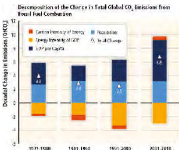
Figure 1.6: Decomposition of the decadal change in total global CO 2 emissions from fossil fuel combustion by four driving factors; population, income (GDP) per capita, energy intensity of GDP and carbon intensity of energy. The bar segments show the changes associated with each factor alone, holding the respective other factors constant. Total decadal changes are indicated by a triangle. Changes are measured in giga tonnes (Gt) of CO 2 emissions per decade; income is converted into common units using purchasing power parities. {WG III SPM.3}
