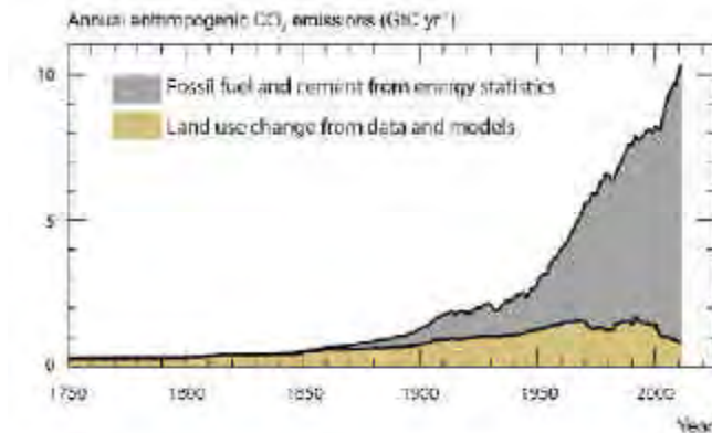
Figure 1.3: Annual anthropogenic CO 2 emissions from fossil fuel combustion, flaring, cement, Forestry and Other Land Use (FOLU) 1750–2011. Emissions are reported in gigatonnes carbon per year (Gt/yr). {WG I Figure TS.4}
