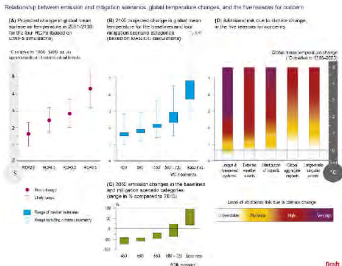
Figure SPM.9: Relationship between emission and mitigation scenarios, global temperature changes, and the five Reasons for Concern (RfC). Temperature changes shown compared with pre-industrial levels. For reference, the extreme right temperature axis shows temperature changes with respect to the 1986-2005 period. Panel a shows projected change in global temperature in 2081-2100 for the four RCPs, based on CMIP5 simulations (see Table 2.1). Panel b shows the projected temperature increase in 2100, calculated using the MAGICC climate model for the baselines and four mitigation scenario categories defined in Chapter WGIII.6, indicating the uncertainty range resulting both from the range of emission scenario projections within each category and the uncertainty in the climate system (data from WGIII.6). Panel c shows the 2050 changes in emissions in the corresponding baselines and mitigation scenario categories (positive changes refer to cases where emissions in 2050 are larger than 2010). For instance, the mitigation scenarios in the 450 category – i.e. with CO 2 e concentration in 2100 between 430 and 480ppm – have emissions in 2050 that are between 41 and 72% percent lower than emissions in 2010 (Table WGIII.SPM.1). Panel d reproduces the five reasons for concerns from WGII Assessment Box SPM.1 Figure 1, using the same temperature axis than Panel a. Risks associated with reasons for concern (from left to right, denoted as RFC1-5 in Article 2 Box) are shown for increasing levels of climate change. The color shading indicates the additional risk due to climate change when a temperature level is reached and then sustained or exceeded. Examples of risks represented by RFC1 include those to coral reefs and the Arctic system; RFC2, includes risks associated with extreme heat; RFC3, regionally differentiated risks to food and water; RFC4, aggregate economic damages and biodiversity loss; RFC5, risk associated with a large sea level rise due to loss of mass from polar ice sheets. Undetectable risk (white) indicates no associated impacts are detectable and attributable to climate change. Moderate risk (yellow) indicates that associated impacts are both detectable and attributable to climate change with at least medium confidence, also accounting for the other specific criteria for key risks. High risk (red) indicates severe and widespread impacts, also accounting for the other specific criteria for key risks. Purple, introduced in this assessment, shows that very high risk is indicated by all specific criteria for key risks. {Ch.19.2} Note the different temperature baselines used in WGII Assessment Box SPM.1 Figure 1. Beyond 2100, temperature, and therefore risk, decreases in most of the lowest three scenarios and increases further in most of the others.
