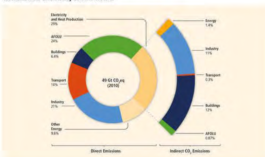
Figure 1.5: Total anthropogenic GHG emissions (GtCO 2 eq/yr) by economic sectors. Inner circle shows direct GHG emission shares (in % of total anthropogenic GHG emissions) of five economic sectors in 2010. Pull-out shows how indirect CO 2 emission shares (in % of total anthropogenic GHG emissions) from electricity and heat production are attributed to sectors of final energy use. “Other Energy” refers to all GHG emission sources in the energy sector as defined in Annex II other than electricity and heat production [A.II.9.1]. The emissions data from Agriculture, Forestry and Other Land Use (AFOLU) includes land-based CO 2 emissions from forest fires, peat fires and peat decay that approximate to net CO 2 flux from the Forestry and Other Land Use (FOLU) sub-sector as described in Chapter 11 of this report. Emissions are converted into CO 2 -equivalents based on GWP 100 6 from the IPCC Second Assessment Report. Sector definitions are provided in Annex II.9. {WGIII Figure SPM.2}
