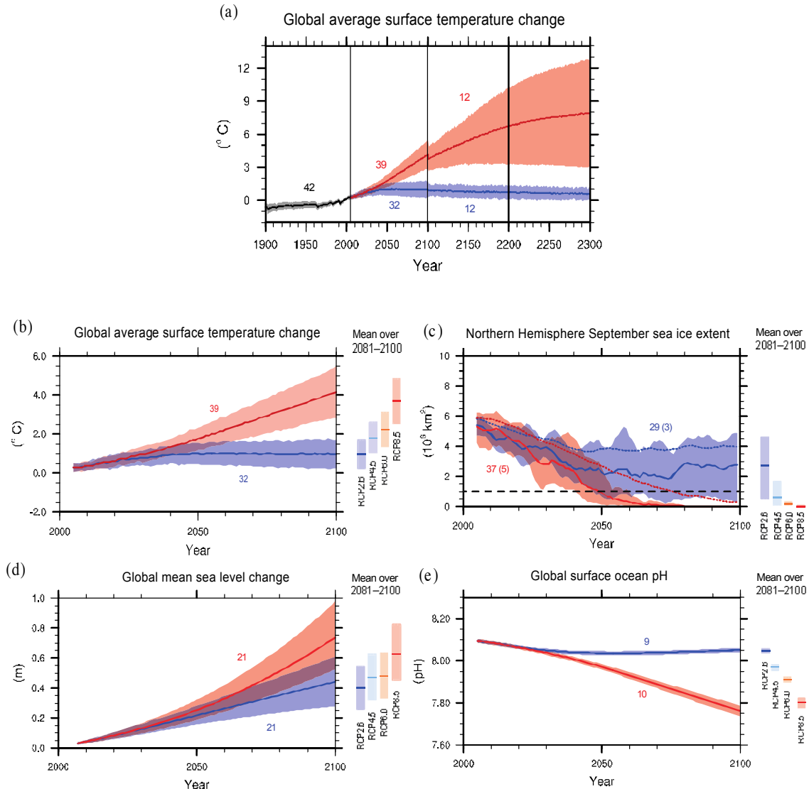
Figure 2.2: CMIP5 multi-model simulated time series from 1900 to 2300 for change in global annual mean surface temperature, (b) Same as (a) but for the 2005-2100 period, (c) Northern Hemisphere September sea ice extent change relative to (5 year running mean). (d) global mean sea level rise, and (e) ocean surface pH. All changes are relative to 1986–2005. Time series of projections and a measure of uncertainty (shading) are shown for scenarios RCP2.6 (blue) and RCP8.5 (red). The mean and associated uncertainties averaged over 2081–2100 are given for all RCP scenarios as colored vertical bars at the right end of each panel. The number of CMIP5 models used to calculate the multi-model mean is indicated. For sea ice extent (c), the projected mean and uncertainty (minimum-maximum range) of the subset of models that most closely reproduce the climatological mean state and 1979–2012 trend of the Arctic sea ice is given (number of models given in brackets). For completeness, the CMIP5 multi-model mean Arctic sea-ice is also indicated with dotted lines. {WGI Figure SPM.7} For sea level (d), based on current understanding, only the collapse of marine-based sectors of the Antarctic ice sheet, if initiated, could cause global mean sea level to rise substantially above the likely range during the 21st century. However, there is medium confidence that this additional contribution would not exceed several tenths of a meter of sea level rise during the 21st century.
